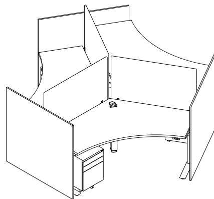
120-DEGREE WORKSTATIONS POD OF 3
