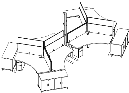
120-DEGREE WORKSTATIONS POD OF 6
